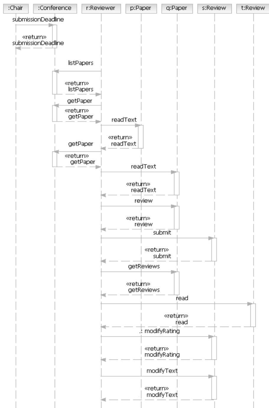
Fig. 3. Sequence diagram
