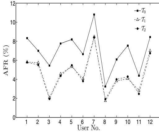
Fig. 3. AFRs of the classifications based on training sets T_0 , T_1 , and T_2
