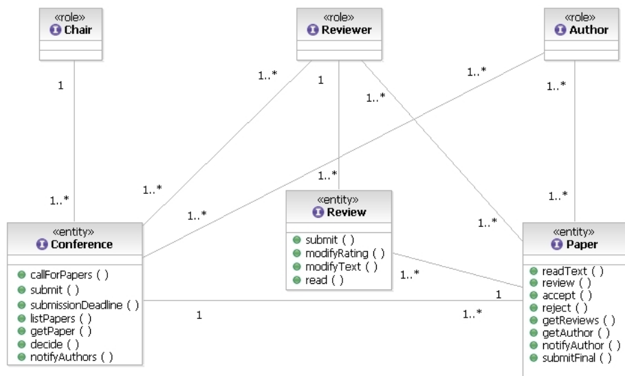
Fig. 2. Class diagram
