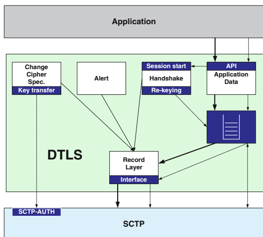
Fig. 6. Structure of SCTP aware DTLS
